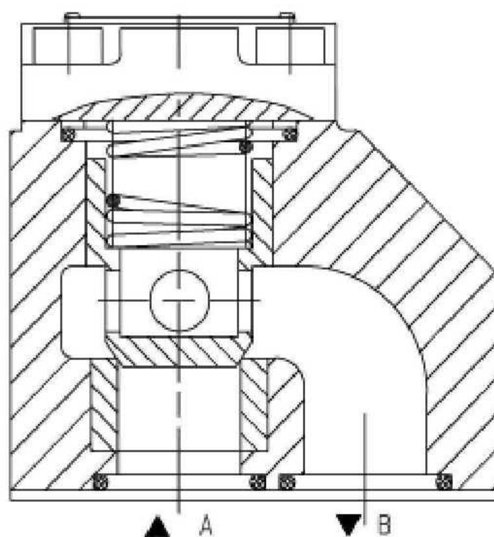
Subplate mounting
